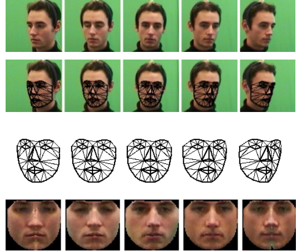
Figure 1. Multi-view dynamic face model. From top to bottom are sample training face images (first row), the landmarks labelled on the images (second row), the estimated 3D shape rotating from -40^\circ to +40^\circ in yaw and with tilt fixed on 0^\circ , and the extracted shape-and-pose-free texture patterns.
