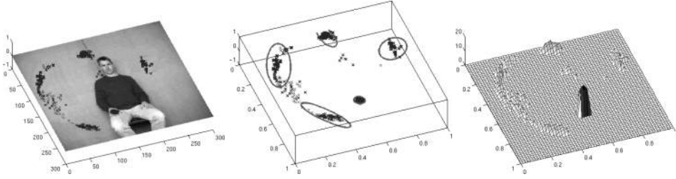
Figure 8: Extracting Rest Positions. Extracted areas with little or no hand motion (left). The distribution approximated by a mixture of Gaussian with 5 mixture components determined using MDL (middle). Probabilities for the rest positions in logarithmic display (right).
