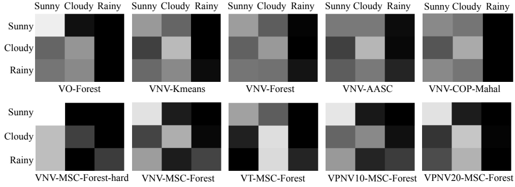
Fig. 7: Weather tagging confusion matrices (TISI dataset).
