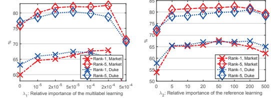
(a) \lambda_1
