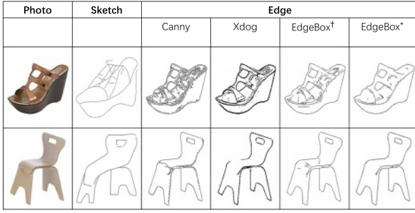
Figure 1: Illustrative examples of edge maps extracted by different algorithms. * : the results reported in [40]. †: our implementation by using the same setting as [40].
