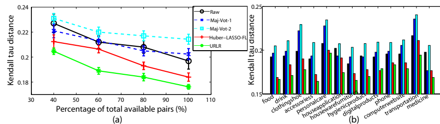
Figure 5. Video interestingness prediction comparative evaluation.
