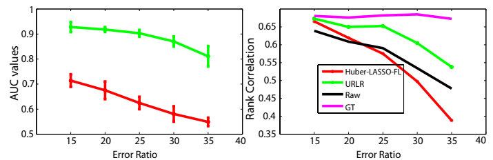
Figure 11. Effect of error ratio. Left: outlier detection performance measured by area under ROC curve (AUC). Right: rank prediction performance measured by rank correlation.
