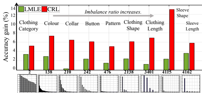
Fig. 8. Performance additional gain over the MTCT by the LMLE and CRL models on 9 X-Domain multi-class clothing attributes [11] with the imbalance ratios (numbers under the bars) increasing from left to right.
